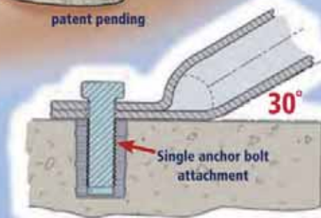
Each longitudinal or lateral Flex Tube is pre-bent to 30 degrees
